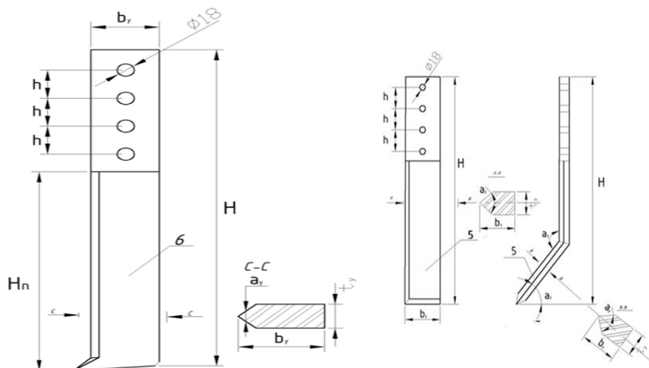
Figure 2. Advanced perforated drainage forming device middle and side work columns
